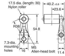
WL-1A118 Nylon Roller: Roller Width: 30 mm
